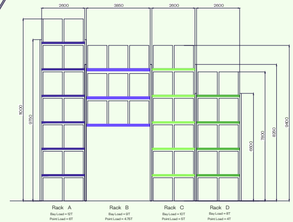
Bay elevation
