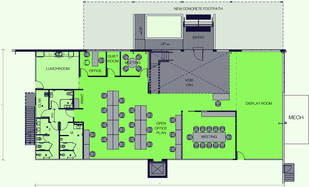
PROPOSED GROUND OFFICE FLOOR PLAN
