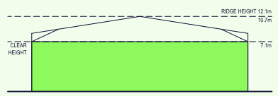
TYPICAL CROSS SECTION
