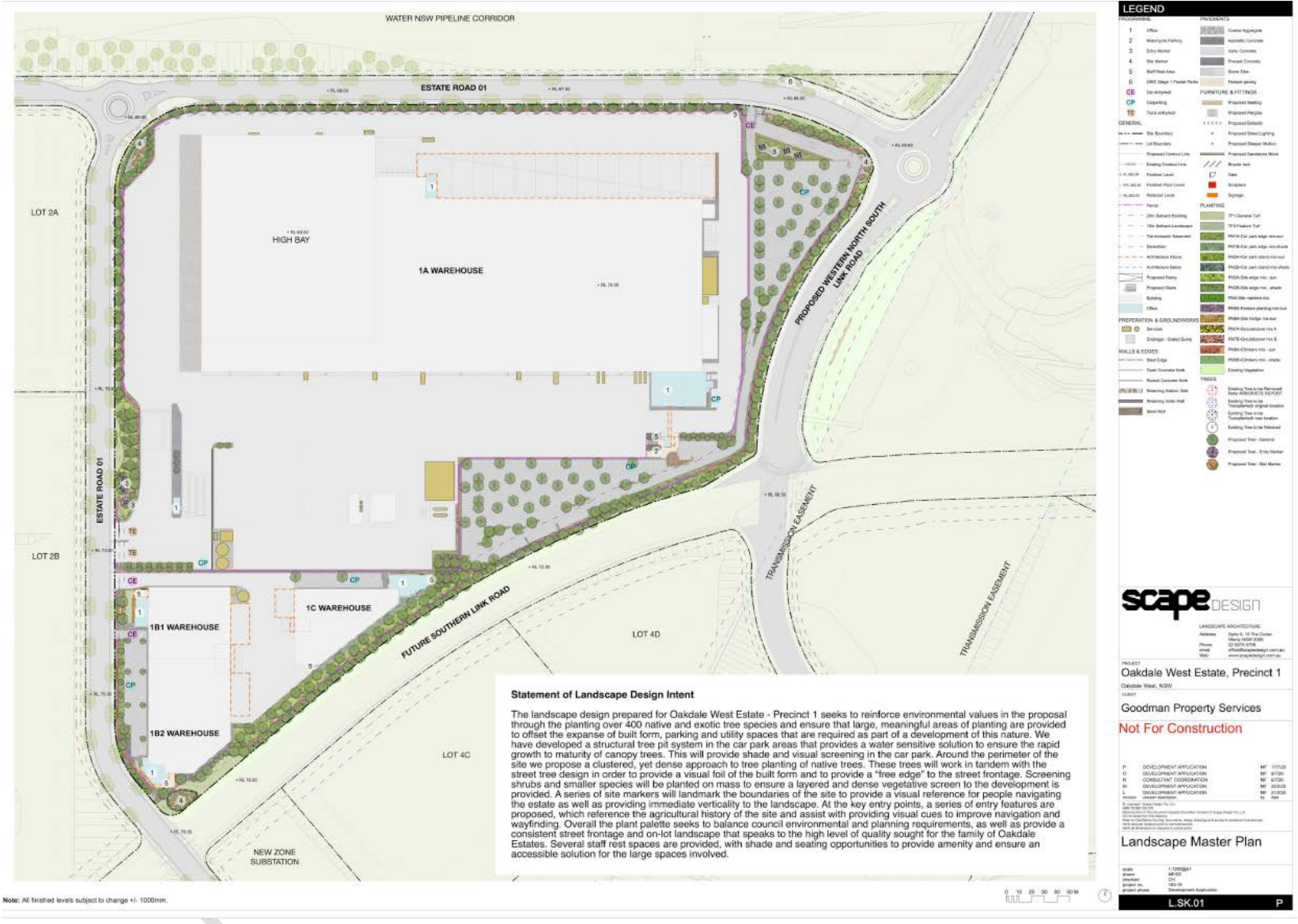
Figure 4: Stage 1 Landscape Plan
