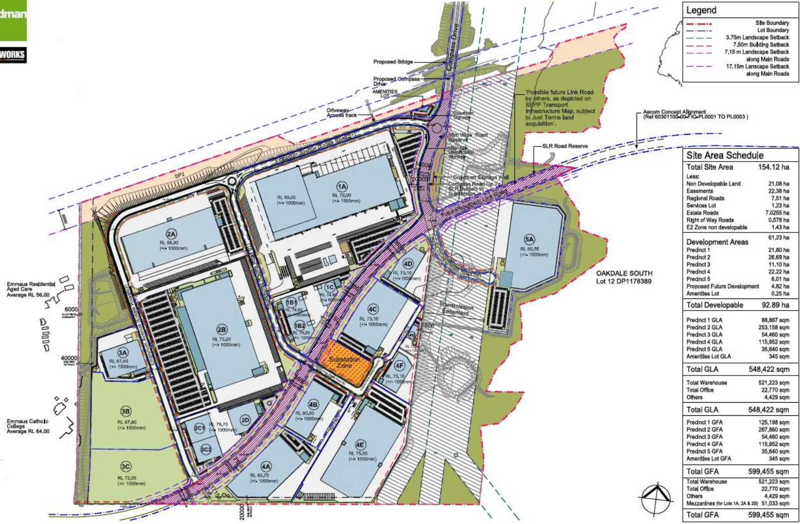
Figure 1: Concept Proposal Layout (MOD 9)
