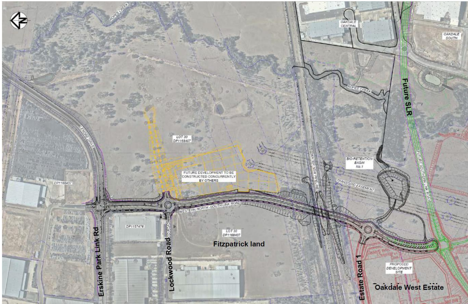
Figure 5: WNSLR
