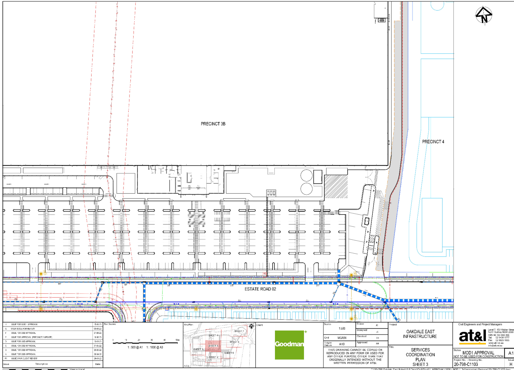
Figure 11: Servicing Plans 3 (Source AT&L; 2023)
