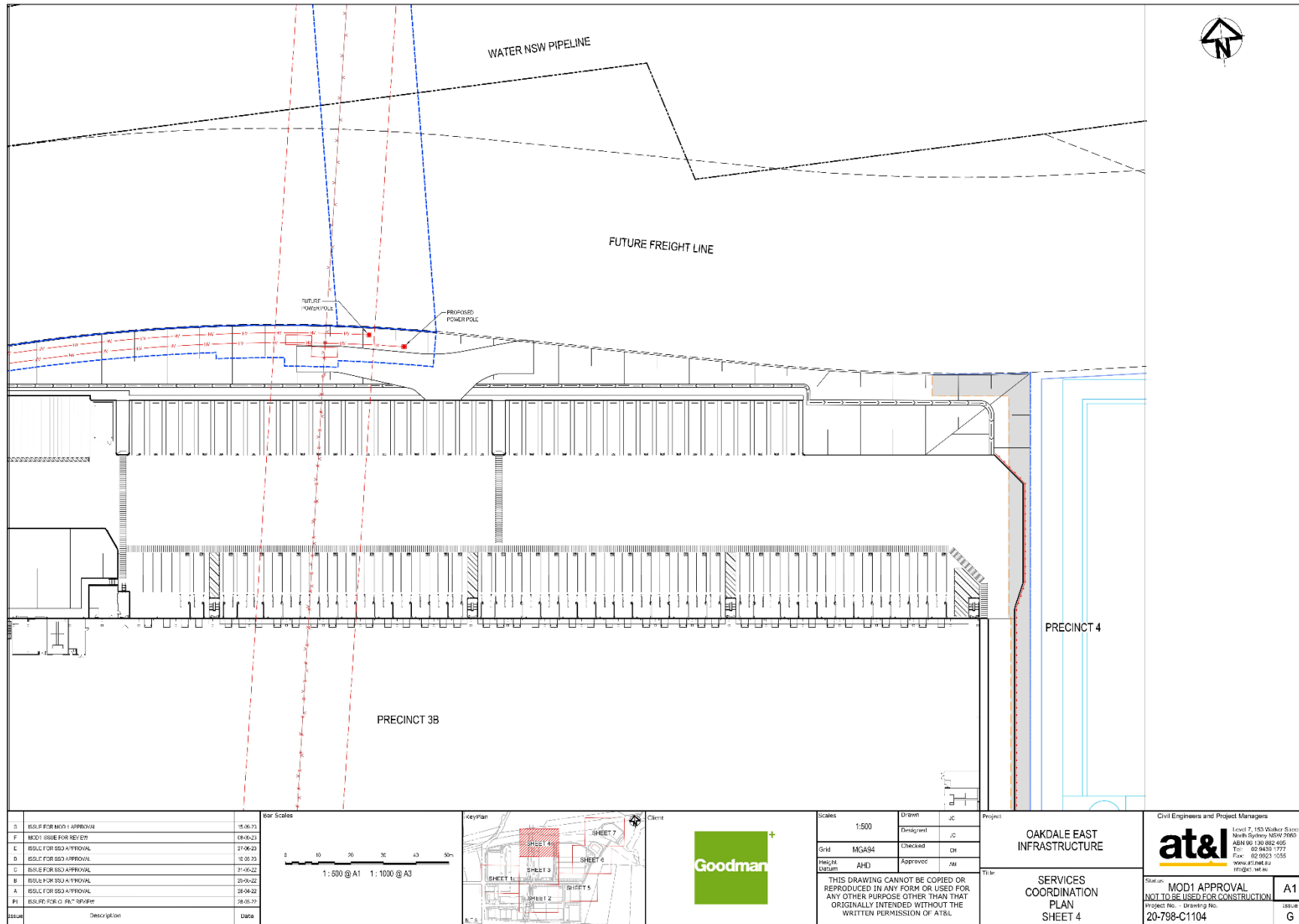
Figure 12: Servicing Plans 4 (Source: AT&L; 2023) .
