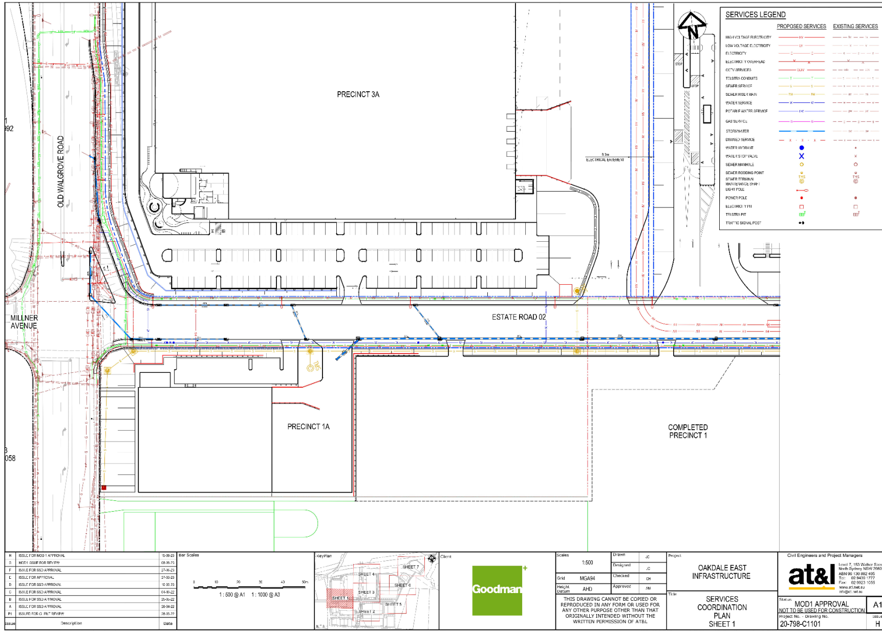
Figure 9: Servicing Plans 1 (Source; AT&L; 2023)
