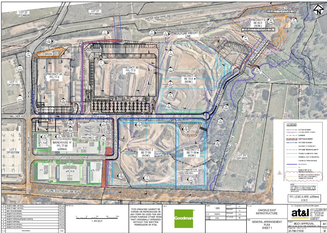
Figure 1: Site general arrangements plan - (Source: AT&L, 2023)
