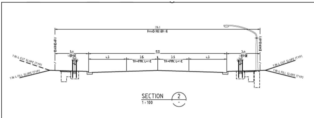
Figure 6: Estate Local Road Typical Cross Section (Source: Ason, 2018)
