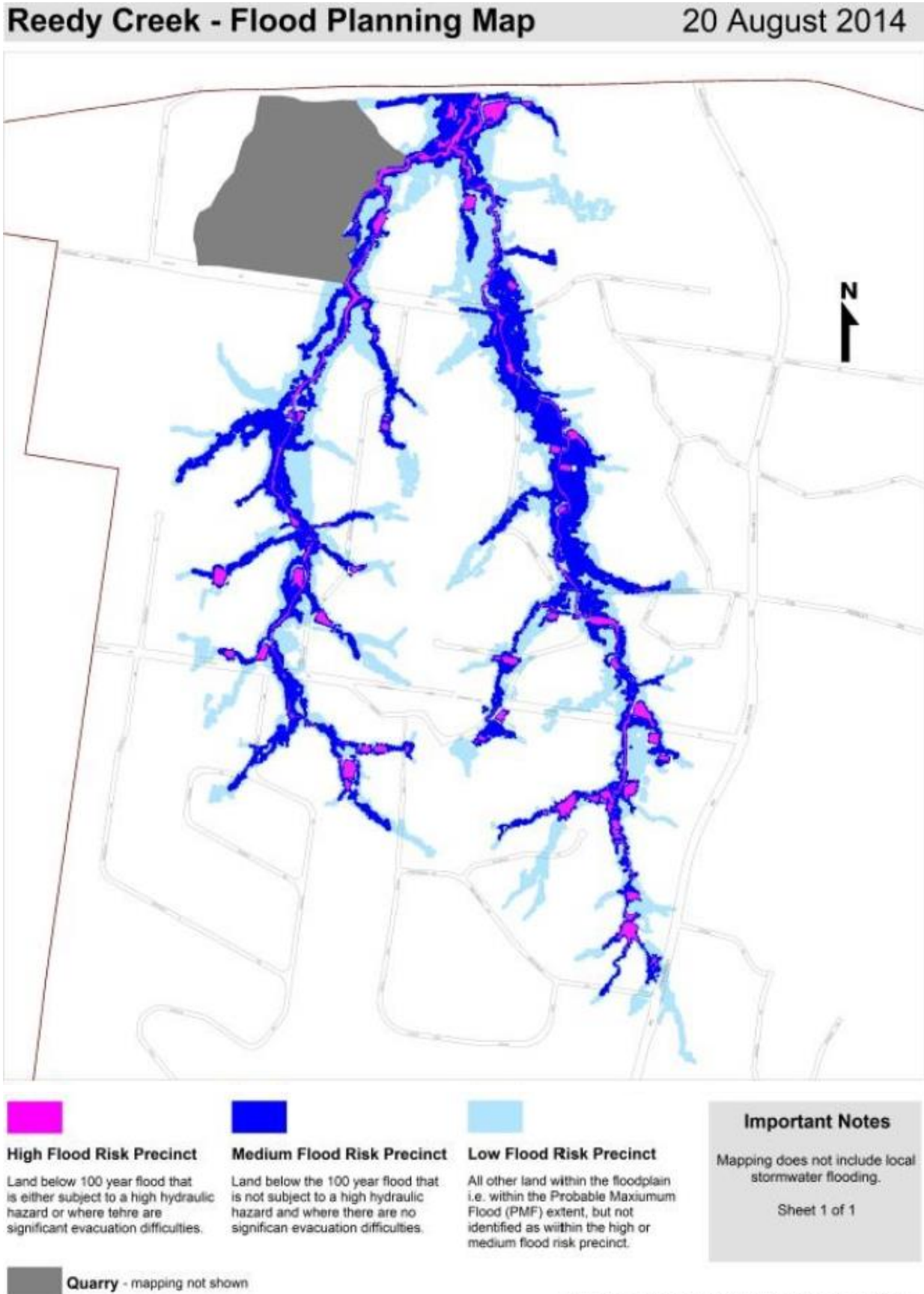
Figure 17: Reedy creek flood mapping
