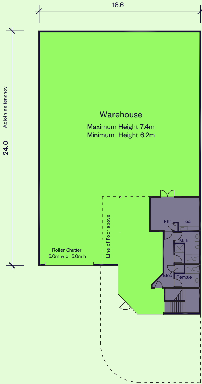
Ground Floor
