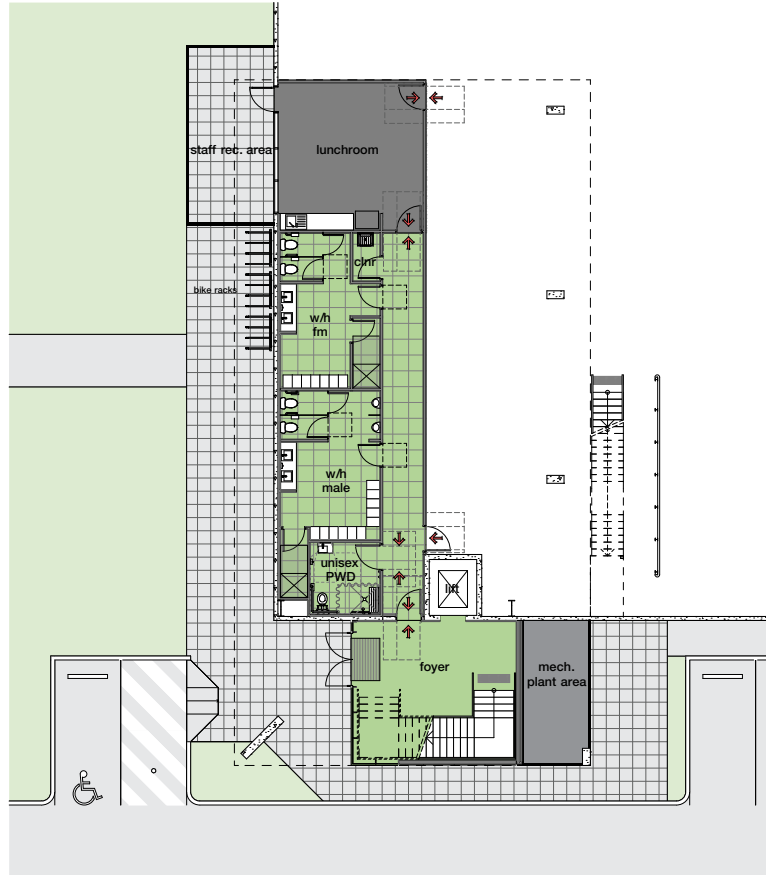
2 tenancy 1 - office ground floor plan SCALE 1:100
