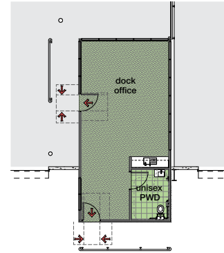
1 tenancy 1 - dock office plan SCALE 1:100
